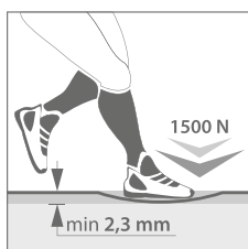
Vertical deformation
